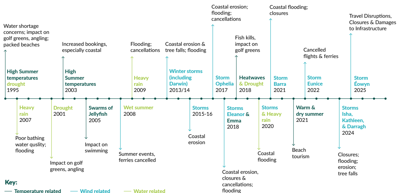
Figure 3.1. Weather events that affected elements of the tourism sector in Ireland 1995-2025.
